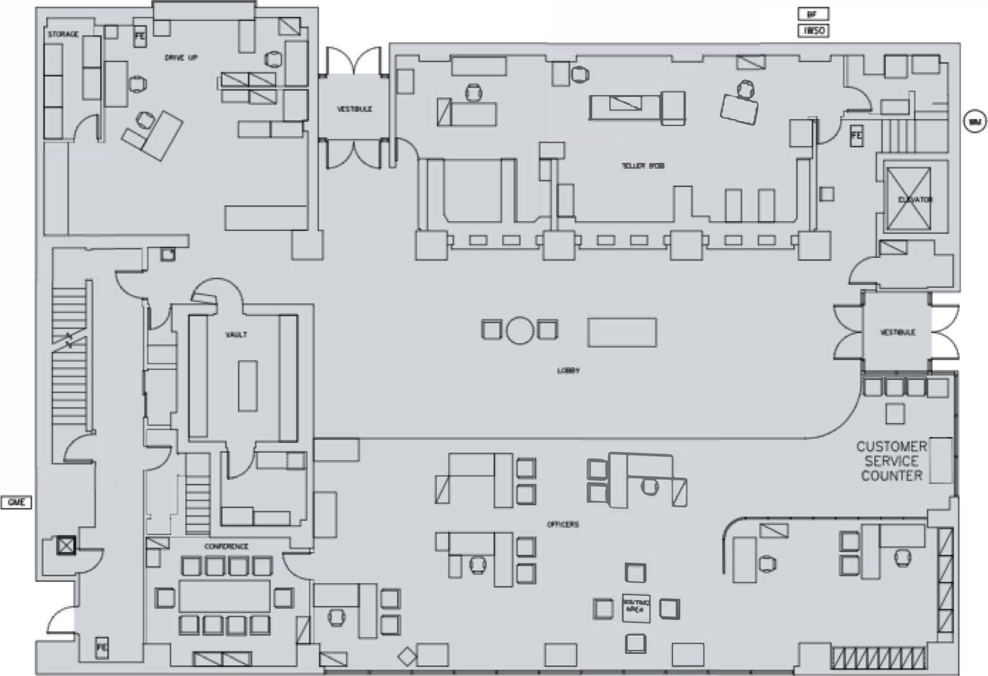
FIRST FLOOR
