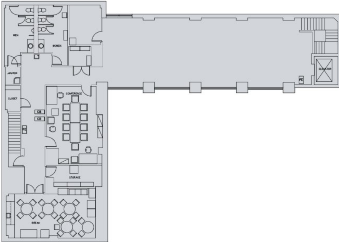
SECOND FLOOR
