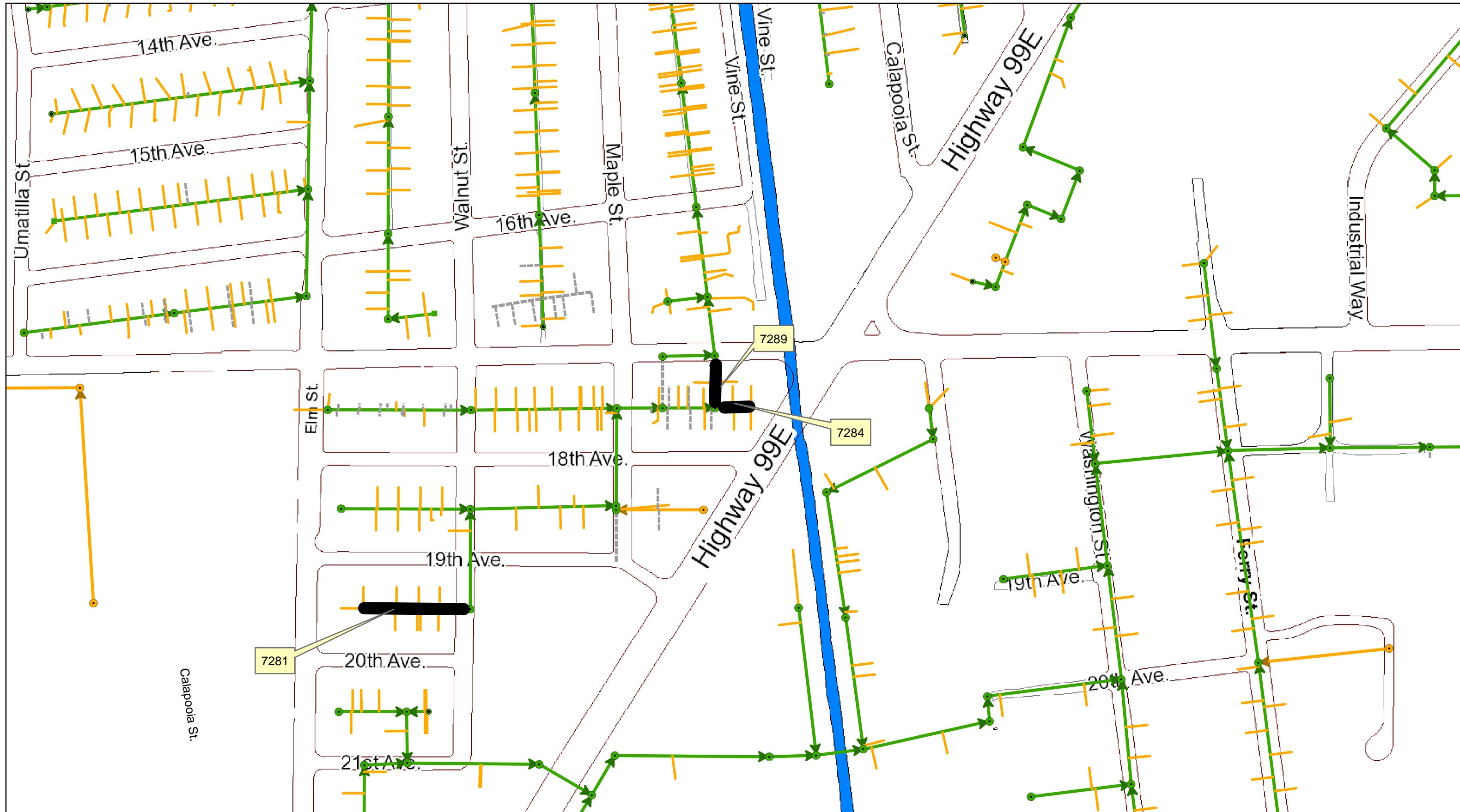
APPENDIX E: SEWAGE BYPASS VICINITY MAP SS-19-01-B Sheet 1 of 4
