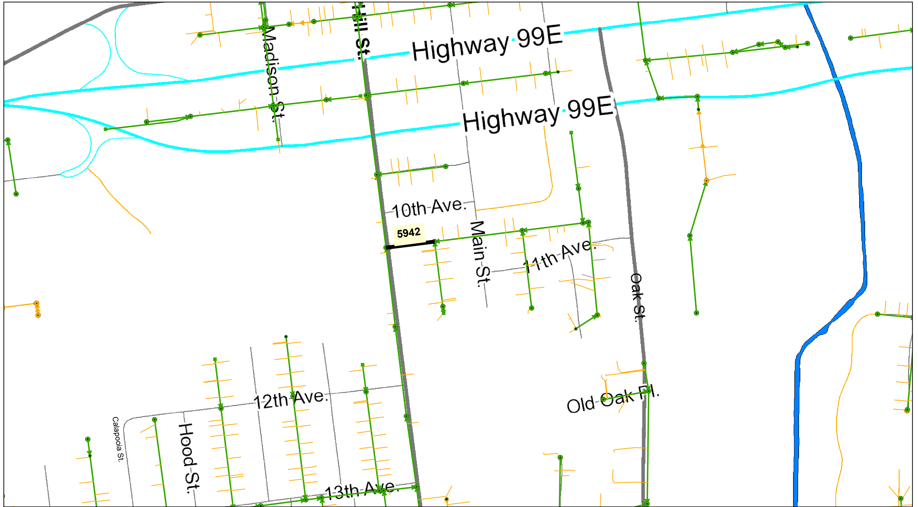
APPENDIX D: SEWAGE BYPASS VICINITY MAP SS-19-03 Sheet 4 of 7
