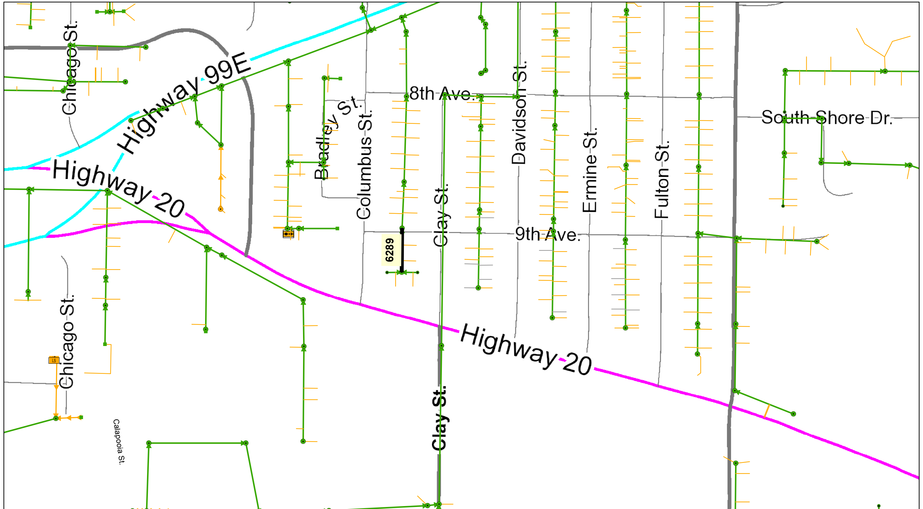
APPENDIX D: SEWAGE BYPASS VICINITY MAP SS-19-03 Sheet 5 of 7
