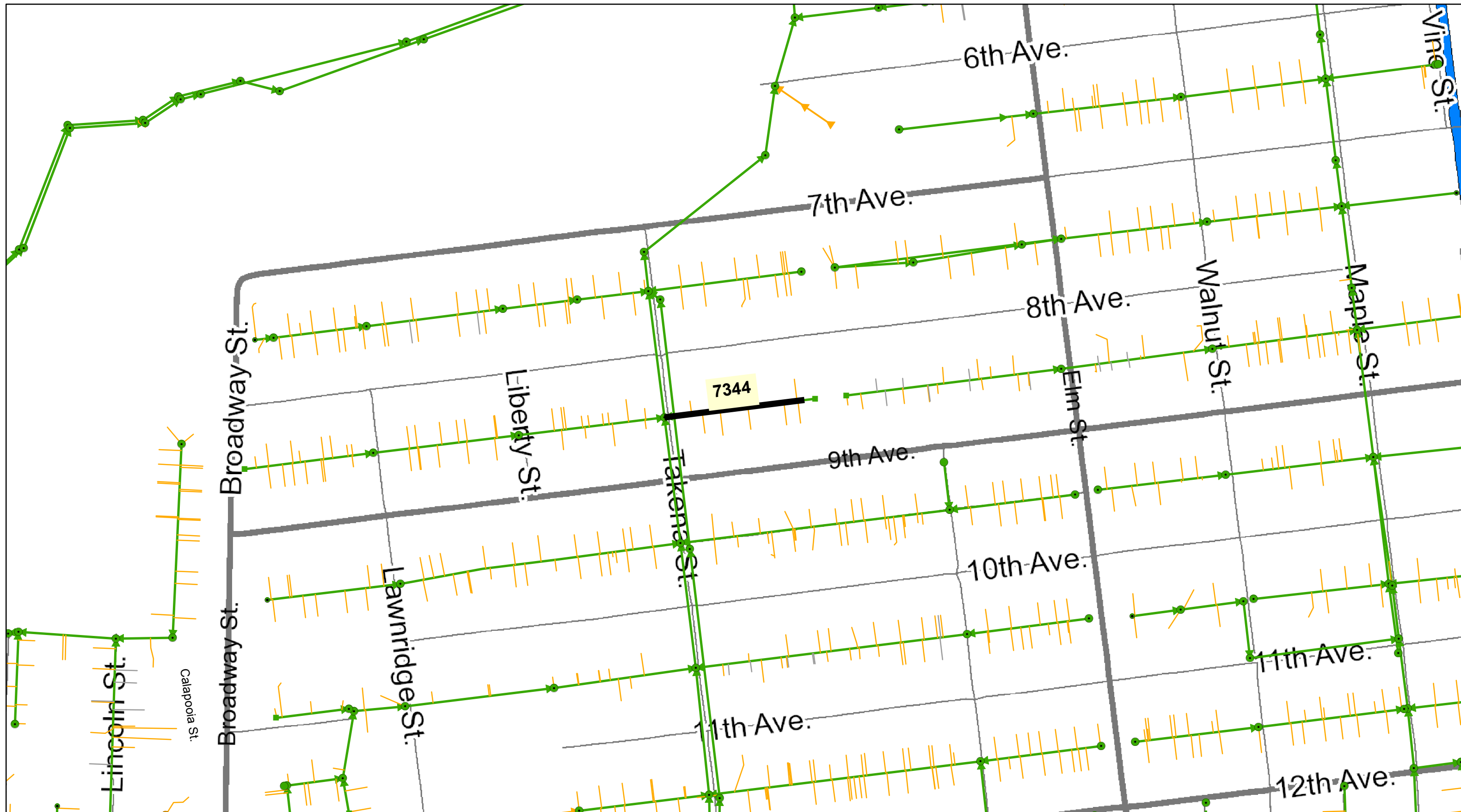
APPENDIX D: SEWAGE BYPASS VICINITY MAP SS-19-03 Sheet 7 of 7
