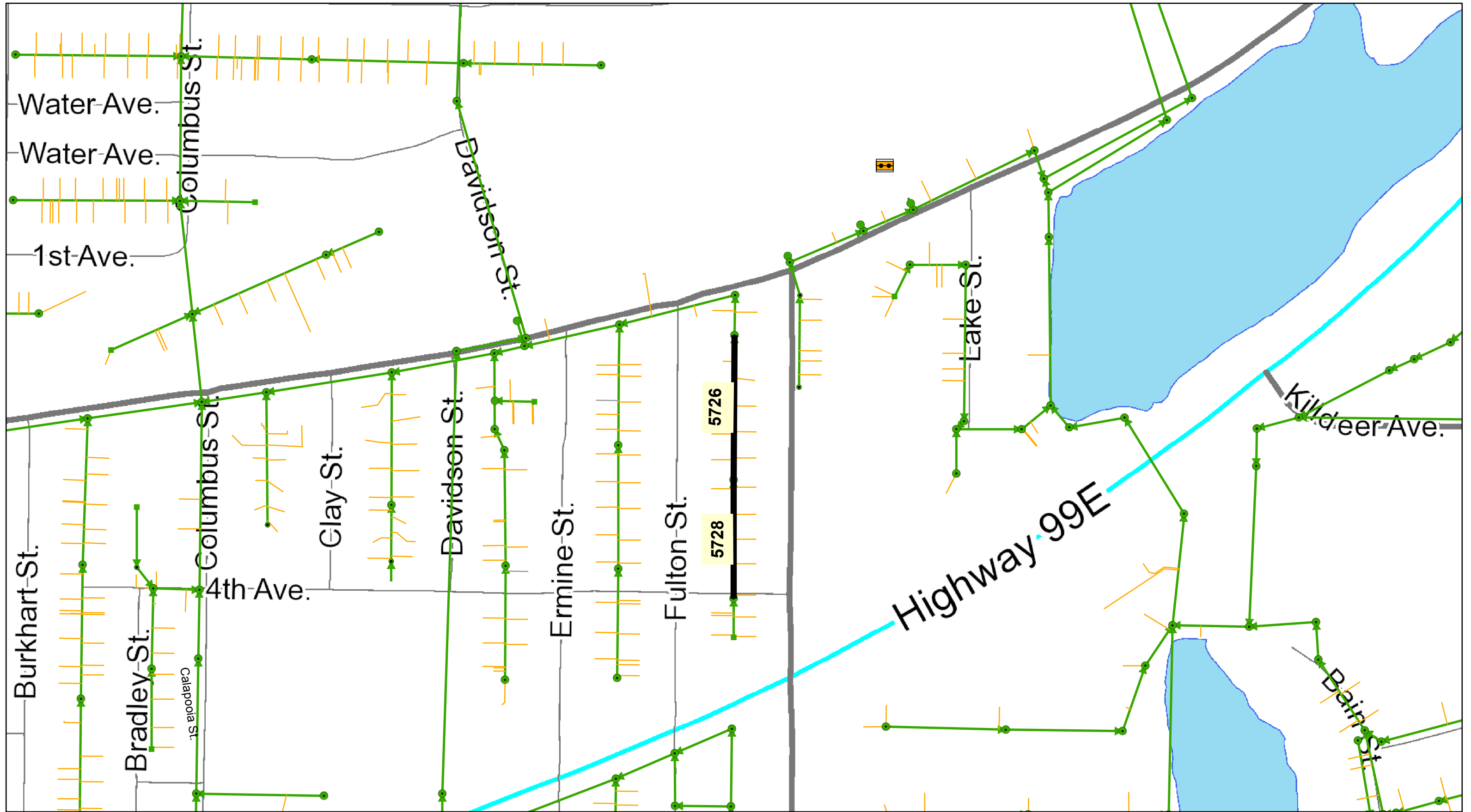
APPENDIX D: SEWAGE BYPASS VICINITY MAP SS-19-03 Sheet 3 of 7
